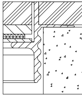
Detail e
