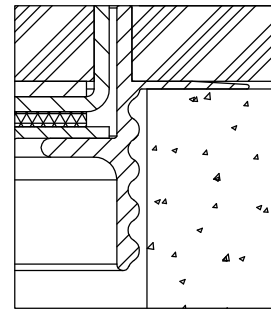
Detail d
