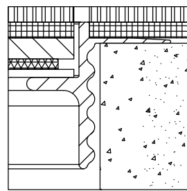
Detail e
