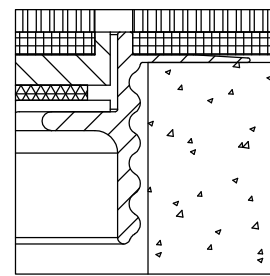
Detail d
